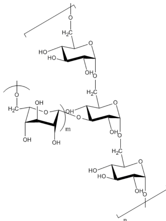
Figure 1. The structure of dextran with branching at C3 [74].
