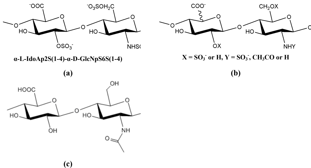
Figure 7. The structure of: (a) the major disaccharide sequence, (b) the minor disaccharide sequence of heparin and (c) the polysaccharide produced by E. coli [85].
