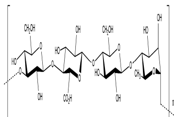
Figure 4. The primary structure of gellan gum [74].
