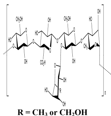
Figure 6. The primary structure of welan gum [74].
