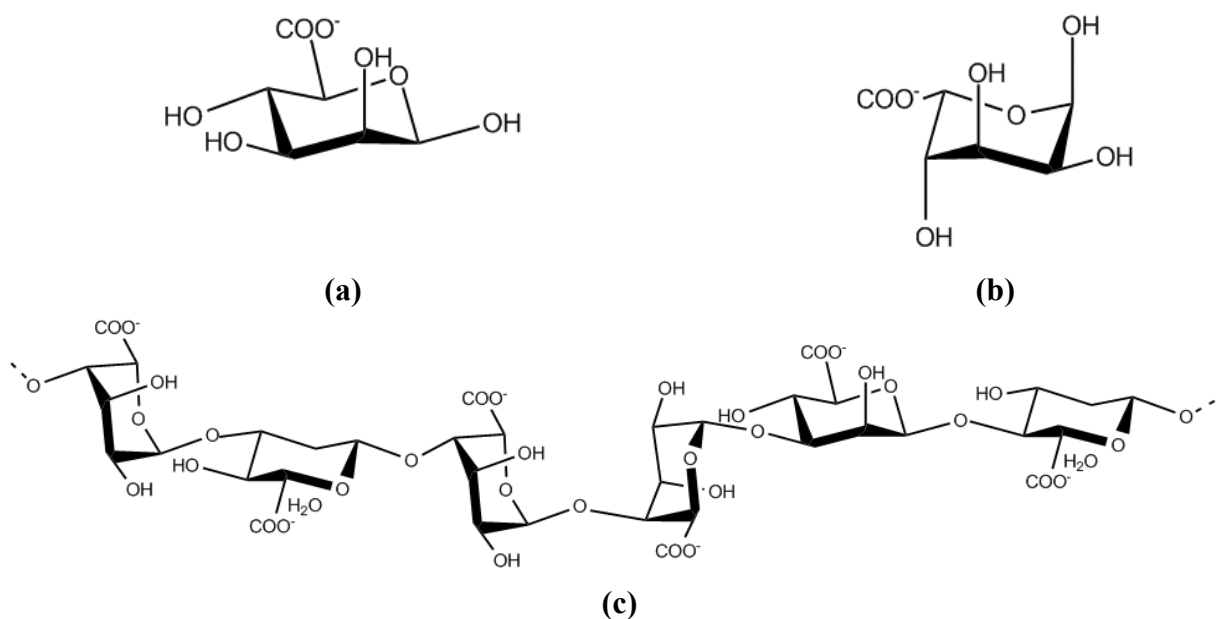
Figure 8. The structure of (a) \beta -D-mannuronic acid, (b) \alpha -L-guluronic acid and (c) alginate [67].
