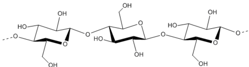
Figure 3. The structure of bacterial cellulose [80].
