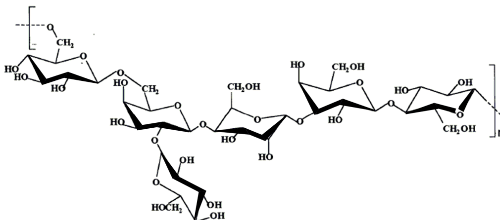
Figure 2. The structure of kefiran, the polysaccharide found in kefir grains [75].
