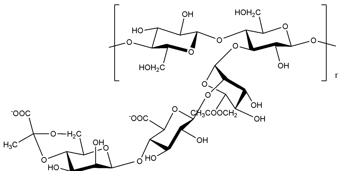
Figure 9. The structure of xanthan [68].
