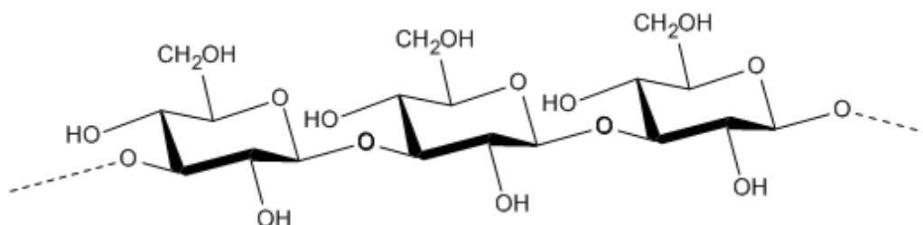
Figure 5. Chemical structure of curdlan [83].
