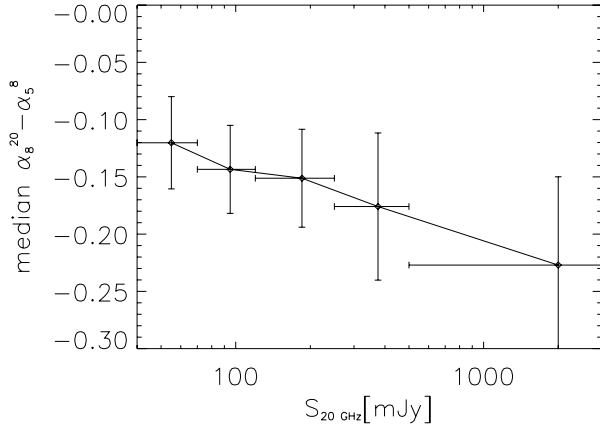
Figure 8. Median values of the spectral curvature \alpha_8^{20} - \alpha_8^8 for different flux density bins.
