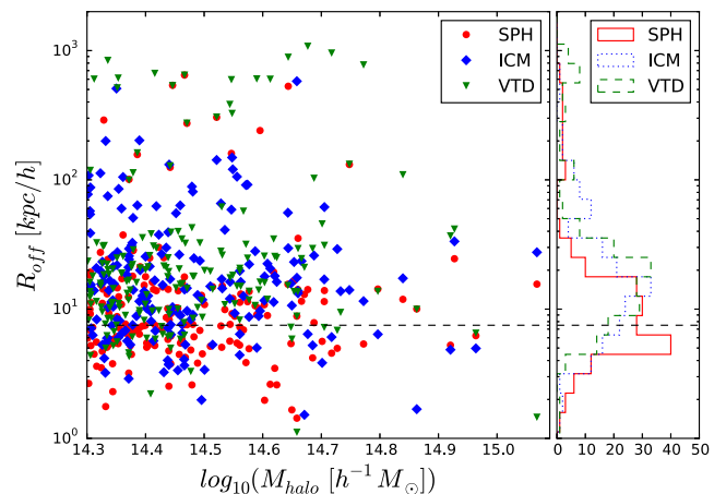
Figure A1. The offsets between three density peak estimators – SPH, Voronoi tessellation density (VTD), and the iterative centre of mass – and the location of the minimum of the gravitational potential, as a function of cluster mass. Red circles, blue diamonds and green inverted triangles correspond to SPH, ICM and VTD estimators respectively. The right-hand panel shows the histograms of the offsets. See the text for further details.
