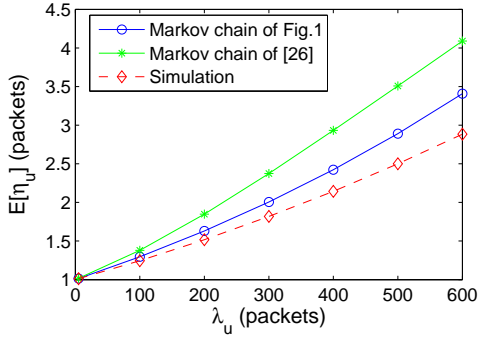
Fig. 2. The average burst size \mathbb{E}[\eta_u] as a function of the arrival rate of an unsaturated source \lambda_u . (Unsaturated stations: Poisson arrivals with rate \lambda_u , N_u = 1 , l_u = 100 Bytes, W_u = 32 , r_u = 7 ; Saturated stations: N_s = 1 , l_s = 1040 Bytes, W_s = 32 , \eta_s = 1 .)
