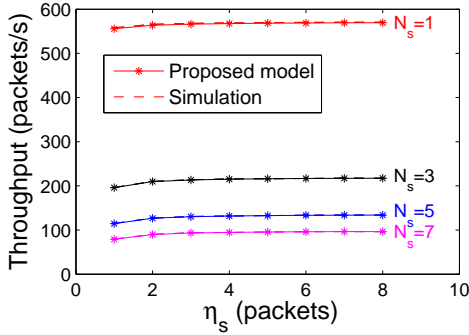
(a) Throughput of a saturated source.
