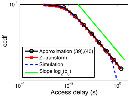
Fig. 7. Distribution of access delay. (Unsaturated stations: Poisson arrivals with rate \lambda = 10 packets/s, N_u = 20 , l_u = 100 Bytes, W_u = 32 , \eta_u = 1 ; Saturated stations: N_s = 6 , l_s = 1040 Bytes, W_s = 32 , \eta_s = 1 .)
