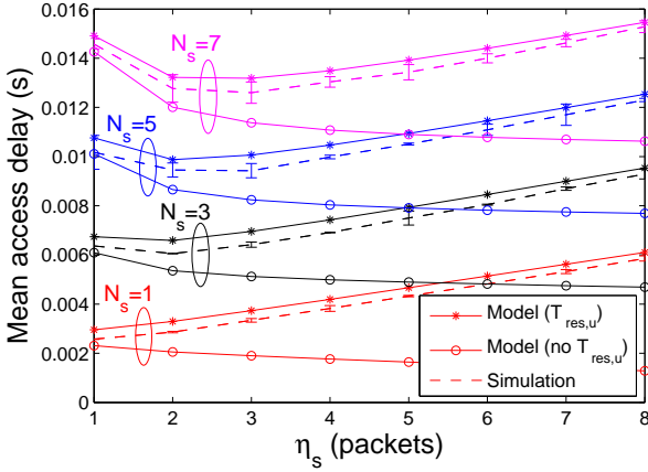
(b) Mean access delay of an unsaturated source
