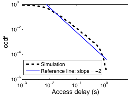
Fig. 8. Access delay distribution of unsaturated sources. (Unsaturated stations: Poisson with \lambda = 10 packets/s, N_u = 1 , l_u = 100 Bytes, W_u = 32 , \eta_u = 1 ; Saturated stations: N_s = 8 , l_s = 1040 Bytes, W_s = 32 , \eta_s = 1 .)
