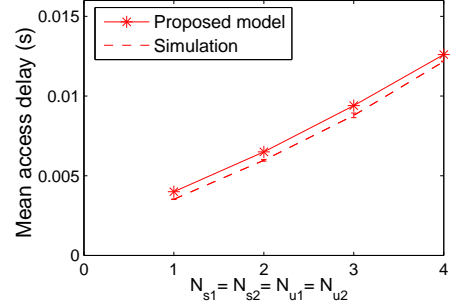
(b) Mean access delay of an unsaturated source of type u1
