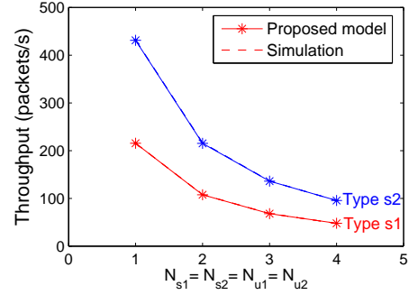
(a) Throughput of saturated sources
