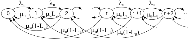
Fig. 1. The transition diagram of queue size of an unsaturated source u .
