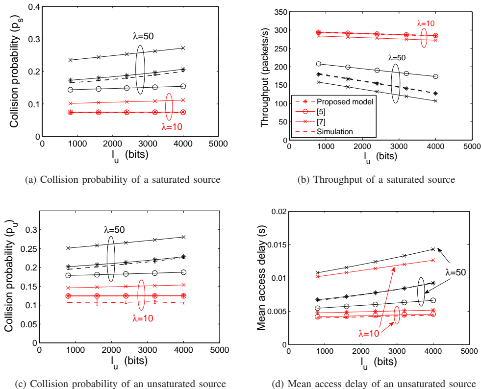
Fig. 4. Collision probabilities, throughput, and mean access delay for DCF, Scenario 2. Figs. 4(b) and 4(d), respectively, show clearly that our model is much more accurate than the models in [5] and [7]. (Unsaturated stations: Poisson arrivals with rate \lambda , N_u = 10 , W_u = 32 , \eta_u = 1 ; Saturated stations: N_s = 2 , l_s = 1040 Bytes, W_s = 32 , \eta_s = 1 .)
