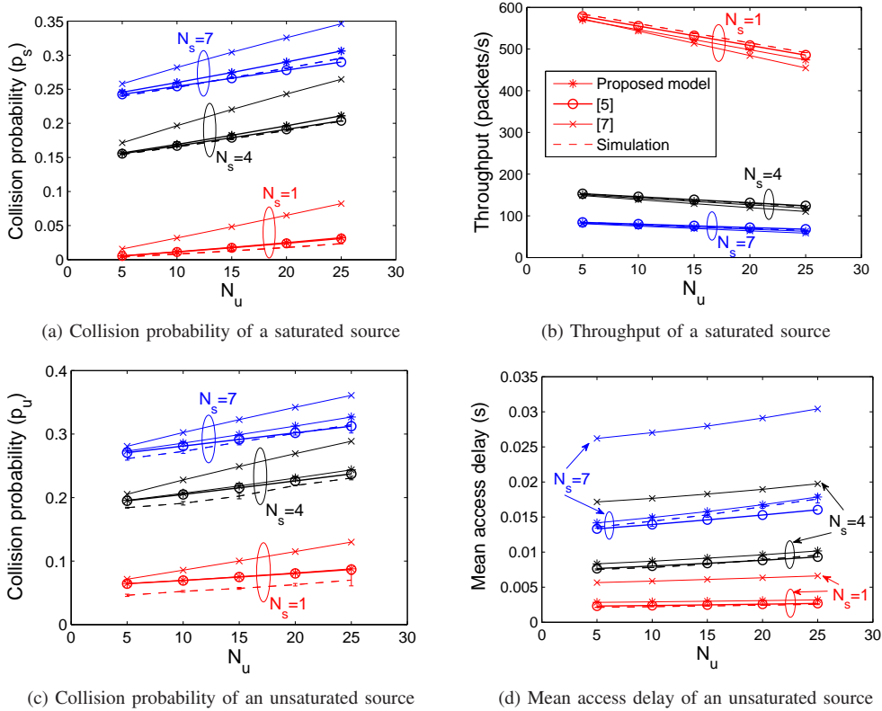
Fig. 3. Collision probabilities, throughput, and mean access delay for DCF, Scenario 1. Figs. 3(a), 3(c) and 3(d) clearly show that our model is much more accurate than the model in [7]. (Unsaturated stations: Poisson arrivals with rate \lambda = 10 packets/s, l_u = 100 Bytes, W_u = 32 , \eta_u = 1 ; Saturated stations: l_s = 1040 Bytes, W_s = 32 , \eta_s = 1 .)
