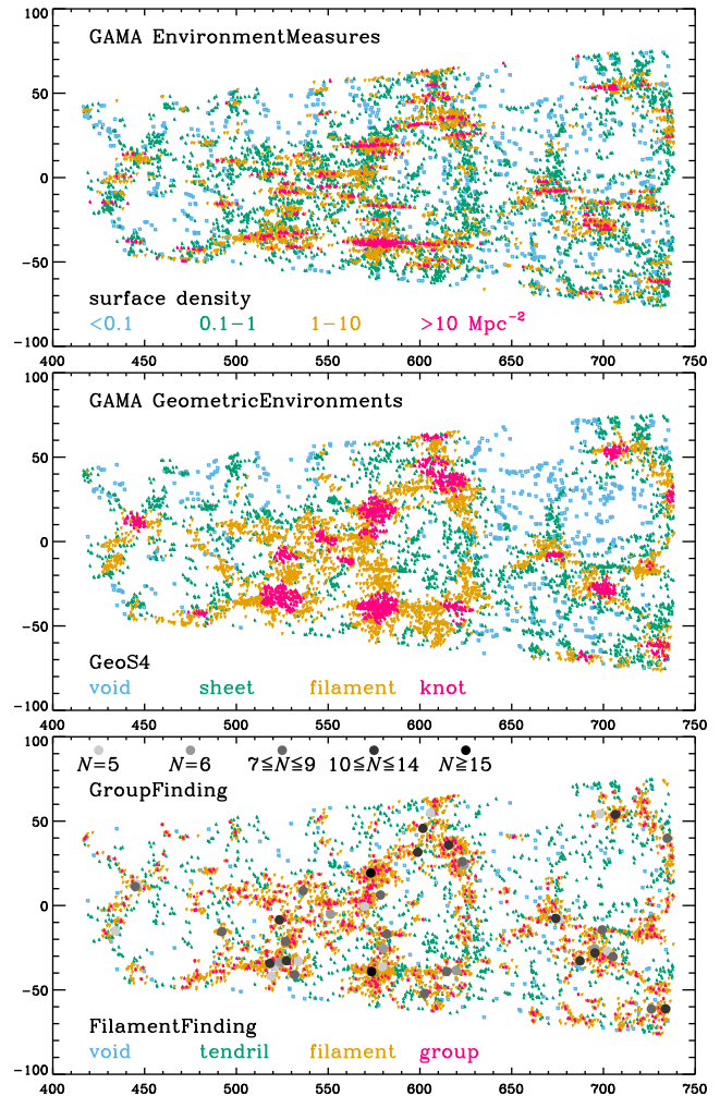
Figure 15. Galaxy distribution in the GAMA G15 field showing different environmental measurements. Galaxies were selected with 0.10 < z < 0.18 and -1^\circ 5 < \text{Dec} < 1^\circ 5 (the two dimensions shown correspond to RA and redshift). Each panel shows the galaxies colour-coded according to environment: top panel, using the fifth nearest neighbour surface density (Brough et al. 2013); middle panel, using the geometric environment classifications (Eardley et al. 2015); lower panel, using the filament-finder classifications (Alpaslan et al. 2014a). The top two panels show a volume-limited sample with M_r < -20.0 mag, while the filament finder uses only galaxies with M_r < -20.55 mag ( h = 0.7 ). In the latter case, the classified groups, from the FoF catalogue (Robotham et al. 2011), used as the starting point of the filament finder, are those with two or more members from the volume-limited sample. Also shown are rich groups shaded according to the number of member galaxies with M_r < -21.0 mag (cf. Fig. 7). Note also the FilamentFinding DMU provides links between galaxies and groups in a filament.
