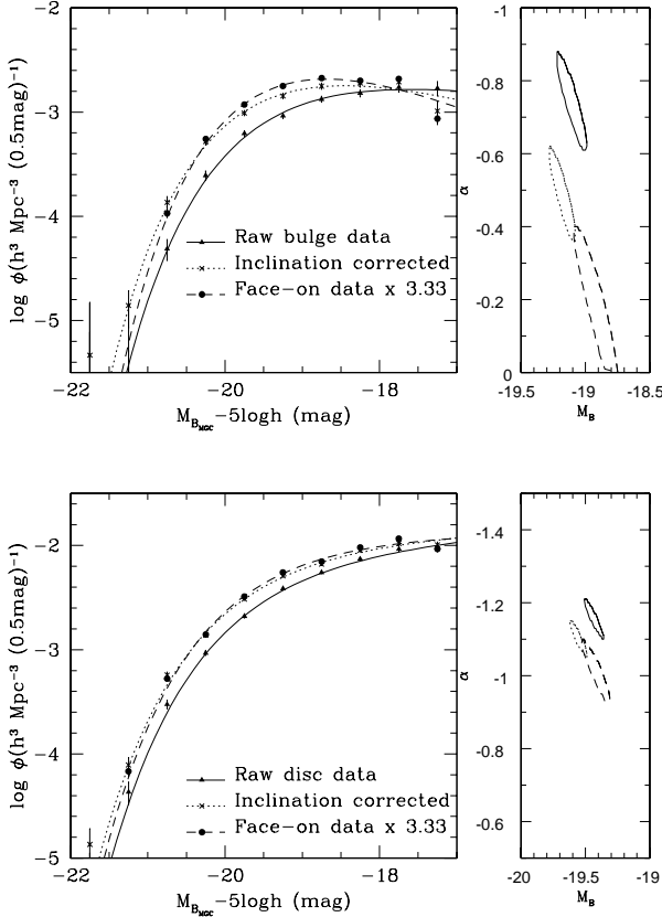
Figure 7. The upper panel shows the bulge luminosity distribution and function before (solid line) and after (dotted line) applying the attenuation–inclination correction. The dashed line shows the luminosity function derived only from face-on [ 1 - \cos(i) < 0.3 ] data and scaled up by a factor of 3.33. The lower panel shows the same for discs. The right panels show the 1\sigma error contours in the M^* - \alpha plane.
