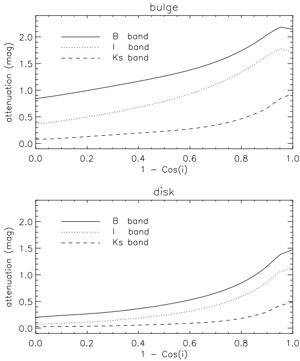
Figure 16. Predicted attenuation-inclination curves in the B , I and K_s bands for the bulge (top panel) and the disk (lower panel) of a galaxy with a central face-on optical depth in the B_{\text{MGC}} -band of \tau_B^f = 3.8 .
