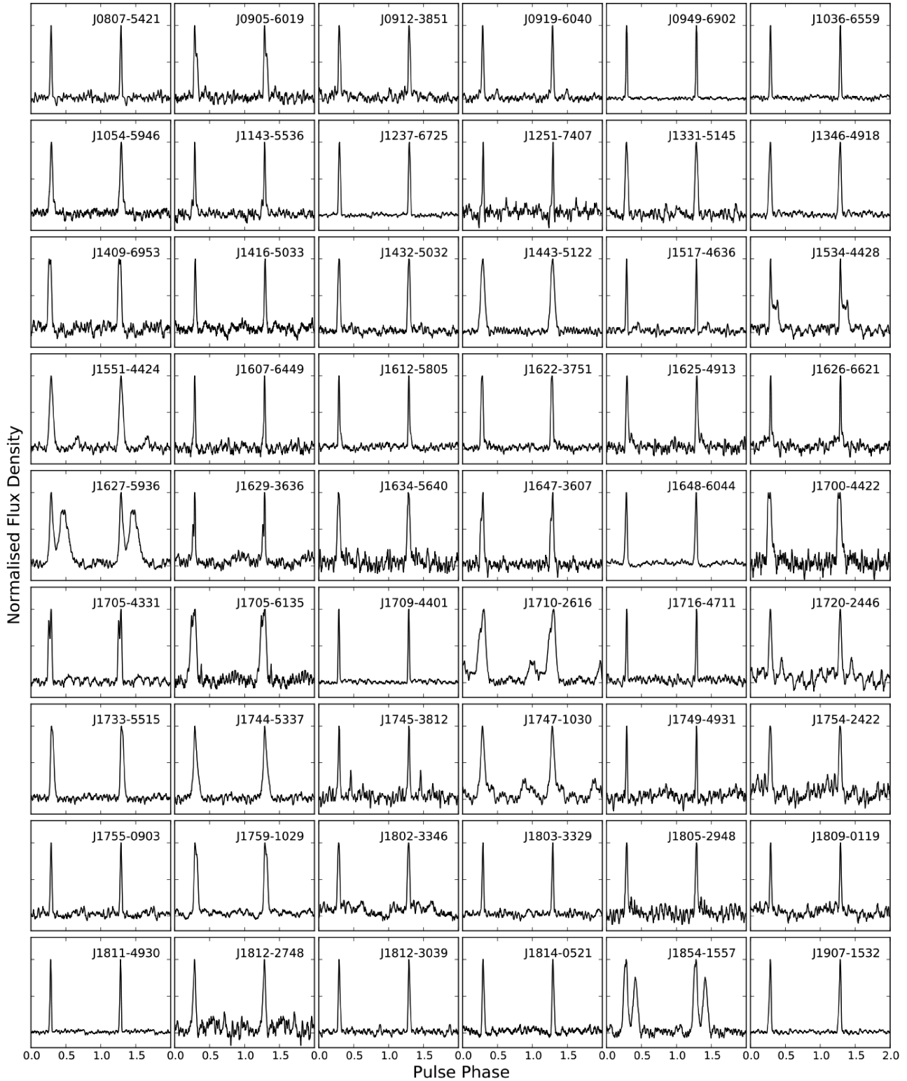
Figure 3. Pulse profiles at an observing frequency of 1.4 GHz for each of the pulsars with a full timing solution, made by summing several timing observations. Profiles are not flux-calibrated, and the amplitudes have all been normalized to one.
