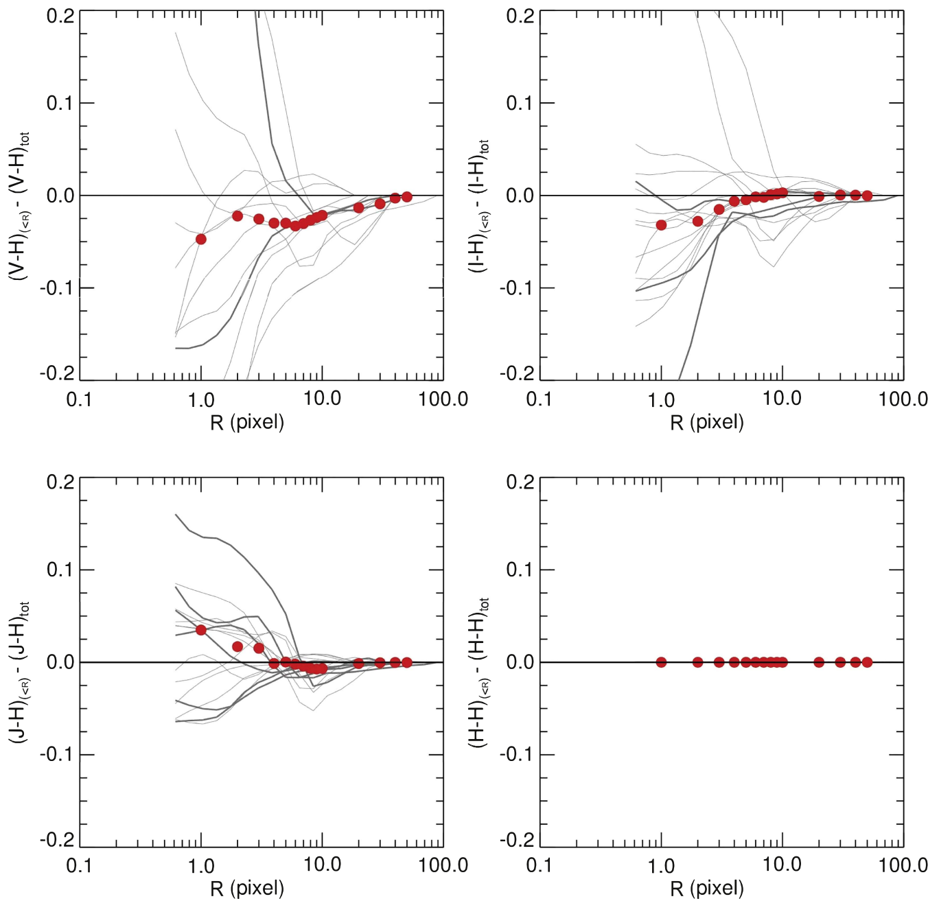
Figure 10. Integrated color differences between H (F160W) and blue bands ( J (F125W), I (F814W), and V (F606W)) for unsaturated stars brighter than 24 mag in the H (F160W) band in the GOODS-S field. Gray lines show individual stars. Red circles show the medians. Stars should have no observed color gradients, so the difference between any two bands should be zero at all radii. This check shows that V and I are under-smoothed so the centers of the stars are bluer than the total colors (i.e., artificially bluer than what they should be). J is over-smoothed so the centers are redder there. At R > 3 pixels, the deviations of the red circles in I and J are almost zero. The deviation in V is larger, but still less than \sim 0.025 mag.
