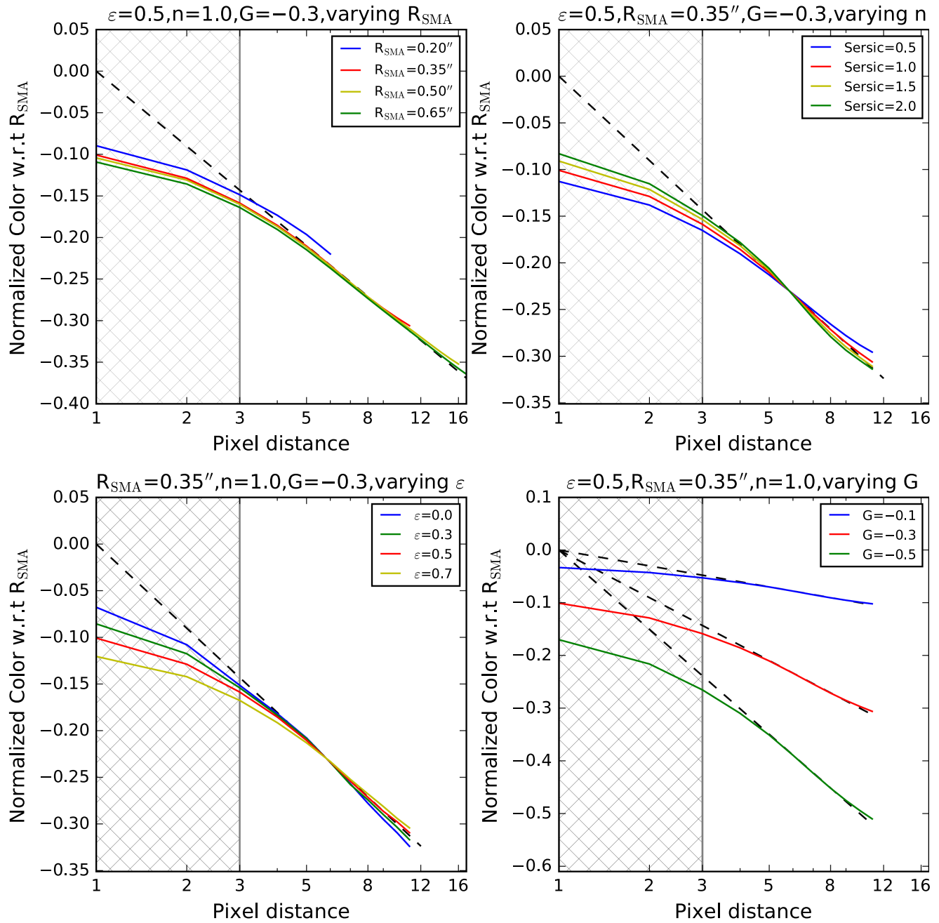
Figure 11. Normalized smeared color gradients in comparison with the intrinsic unit logarithmic gradients ( G ) for mock galaxies with different R_{\text{SMA}} , ellipticity ( \epsilon ), and Sérsic index. Zero points are all fixed at R_{\text{SMA}} .
