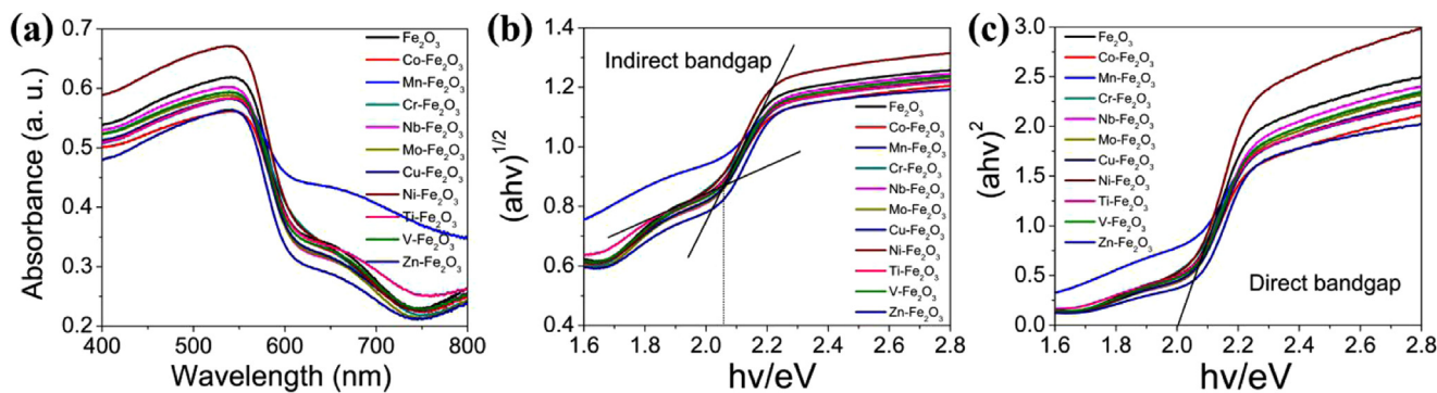
Fig. 5. (a) UV-vis spectra; (b) indirect and (c) direct transitions: (\alpha h\nu)^{1/2} and (\alpha h\nu)^2 vs. (h\nu) of non-doped and TM-doped \text{Fe}_2\text{O}_3 .
