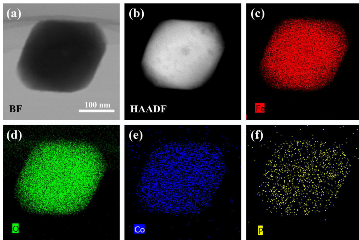
Fig. 4. (a) Bright field (BF), (b) high-angle annular dark field (HAADF) images and (c-f) EDS elemental mapping of Co-doped \text{Fe}_2\text{O}_3 nanoparticles.
