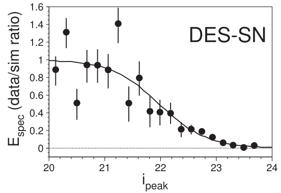
Figure 4. E_{\text{spec}} versus i_{\text{peak}} for DES-SN sample. Filled circles are data/sim ratios, with error bars from Poisson uncertainties on the best-fitting model curve. The simulation includes the first two trigger stages ( E_{\text{spec}} = 1 ), uses the G10 scatter model, and is scaled to match the data statistics for the brightest events. Smooth solid curve is a fit that defines E_{\text{spec}} in the simulation, and max E_{\text{spec}} = 1 is an arbitrary normalization.
