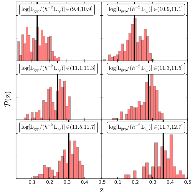
Figure 6. Redshift distributions of the GAMA groups used in this paper in the six r -band luminosity bins. The group luminosity increases from left to right and from top to bottom. The solid vertical black lines indicate the median of the distributions.
