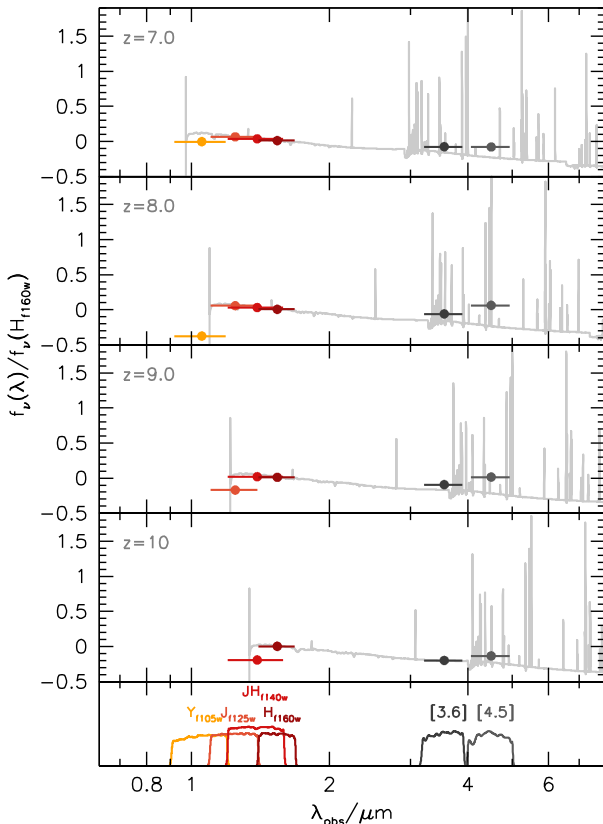
Figure 1. Relative observed NIR photometry of a model star-forming galaxy at z \in \{7, 8, 9, 10\} highlighting the bands available to measure the rest-frame UV-continuum slope. At z > 9.6 , the Spitzer /IRAC [3.6] band can be combined with the H_{f160w} band to measure the UV-continuum slope over a large wavelength baseline, minimizing its uncertainty. At z \sim 8 only the JH_{f140w} and H_{f160w} bands are uncontaminated by the Lyman \gamma break providing only a small wavelength baseline and leaving the uncertainty on the observed UV-continuum slope very large.
