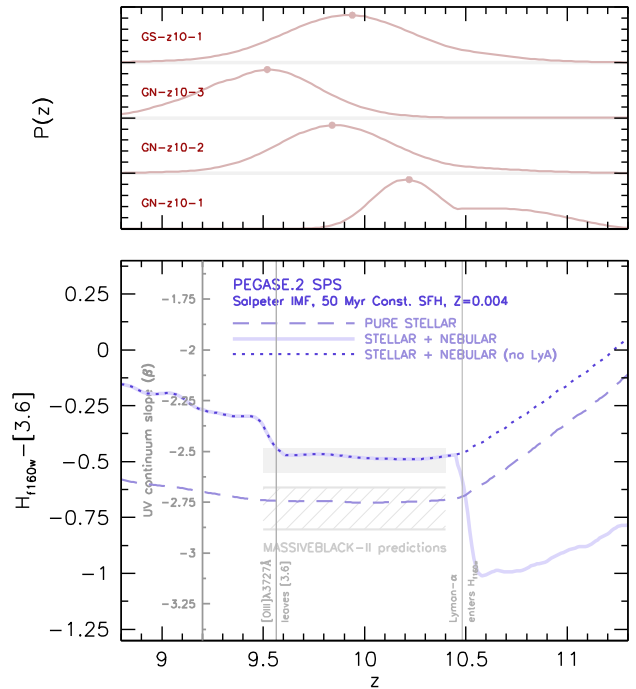
Figure 6. lower-panel: the sensitivity of the H_{f160w} - [3.6] colour (our proxy for the UV-continuum slope) to the redshift for a stellar population which has been constantly forming stars for 50 Myr (with Z = 0.004 , i.e. \approx 1/5 Z_{\odot} ). The three lines show the result of different nebular emission scenarios: (dashed) f_{\text{esc}} = 1 (i.e. pure stellar), (solid) f_{\text{esc}} = 0 , and (dotted) f_{\text{esc}} = 1 but with Lyman \alpha suppressed. The predictions from MassiveBlack-II are shown by the shaded horizontal bands. upper-panel: the redshift probability distributions of the four bright z \sim 10 candidates.
