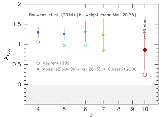
Figure 9. The evolution of the rest-frame UV attenuation A_{1500} inferred from observations of the UV-continuum slope in bright z \in \{4, 5, 6, 7, 10\} star-forming galaxies. Both the attenuation calculated using the Meurer et al. (1999) relation and combining the Calzetti et al. (2000) attenuation curve with the MASSIVEBLACK predictions are shown.
