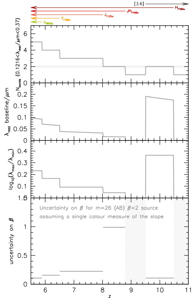
Figure 2. Top panel – the number of Hubble /WFC3 ( Y_{f098m} , J_{f125w} , JH_{f140w} , and H_{f160w} ) and Spitzer /IRAC ([3.6]) bands probing the rest frame 1216 < \lambda_{\text{rest}}/\text{\AA} < 3700 UV continuum as a function of redshift. Second panel – the rest-frame UV wavelength baseline accessible by Hubble /WFC3 and Spitzer /IRAC observations as a function of redshift. Third panel – the ratio of the mean wavelength of the bluest and reddest filters to probe the rest-frame UV continuum. The arrows at the top denote the redshift range over which an individual band probes the rest frame 1216 < \lambda_{\text{rest}}/\text{\AA} < 3700 UV continuum. Bottom panel – the expected uncertainty on the measurement of \beta as a function of redshift. This assumes a \beta = -2 , m = 26 source, for which \beta is measured from the colour providing the longest usable wavelength baseline.
