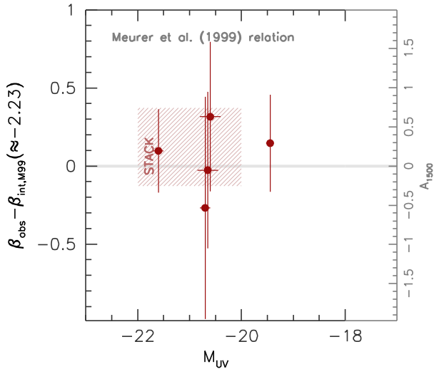
Figure 7. The inferred rest-frame UV attenuation A_{1500} (right-hand axes) assuming the Meurer et al. (1999) relation.
