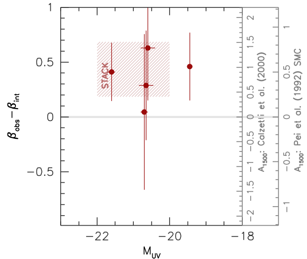
Figure 8. The inferred rest-frame UV attenuation A_{1500} (right-hand axes) assuming the intrinsic slope predicted by MASSIVEBLACK along with the Calzetti et al. (2000) starburst and Pei (1992) SMC dust curves.
