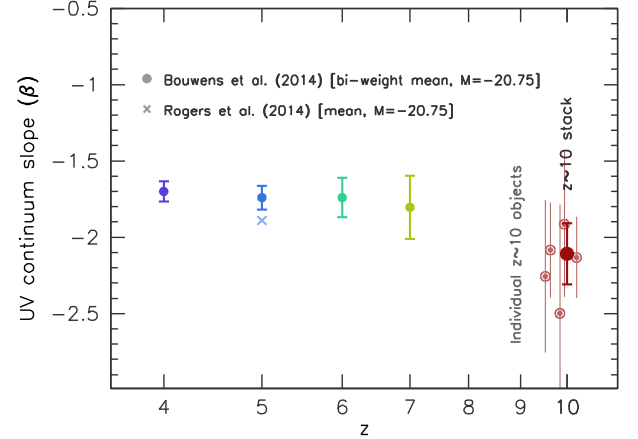
Figure 4. The observed UV-continuum slope as a function of redshift for candidate high-redshift ( z = 4-10 ) star-forming galaxies. Results at z = 4-7 are based on the bi-weight mean of galaxies with M_{1500} \approx -20.75 from Bouwens et al. (2014a).
