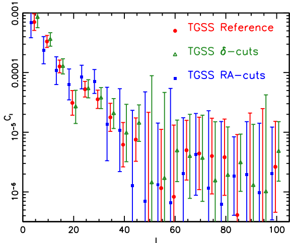
Fig. A.3. Angular power spectrum of the Reference sample (red dots) compared to that of a subsample of TGSS sources in the region -20^\circ < \delta < +60^\circ (green triangles) and of a subsample of TGSS sources in the RA-range [200^\circ, 280^\circ] (blue squares). Error bars represent Gaussian errors. A small horizontal offset has been applied to the green triangles and blue squares to avoid overcrowding.
