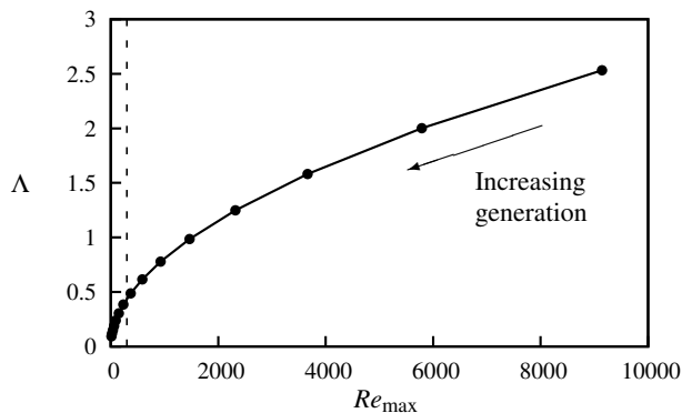
Figure 5: Values of Re_{max} and \Lambda for each generation from 1 to 15 of an example infant airway, using the scaling of Grotberg [2]. Each point represents an airway generation. Practically all generations are approaching the low \Lambda regime, and generations 8 and 9 are close to the optimum value of Re_{max} for maximizing flux (marked with the dashed line) according to the data plotted in figure 2(c).
