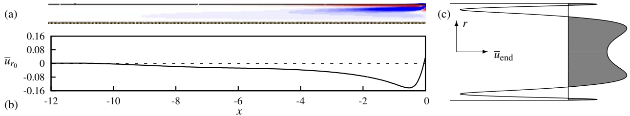
Figure 3: Example measurements of the mean flow for Re_{\max} = 800 , \Lambda = 2.24 . (a) Contours of mean normalised vorticity \Omega = \omega D / U (where \omega is the vorticity with vector out of the plane of the page) in the upper half of the centre plane. Blue/red contours represent positive/negative vorticity. Contour levels are between \Omega = \pm 1 . (b) Mean axial velocity on the centre line of the pipe, near the free end. Note that for the length scale x = 0 is at the free end of the pipe, and x is made non-dimensional with D . (c) The mean velocity profile across the end of the pipe, with the shaded region showing the portions used to find the mean recirculating flux.
