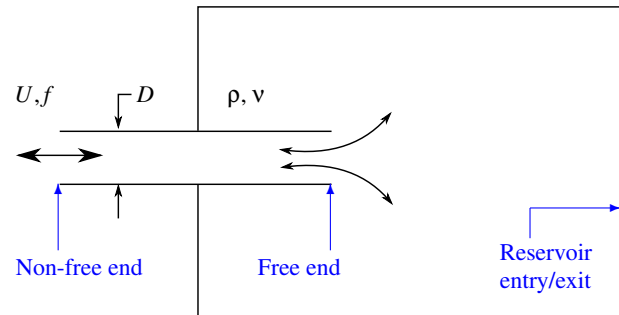
Figure 1: A schematic of the basic problem setup investigated. A time-dependent boundary condition is applied at the non-free end, and the free end acts as an exit/entry to/from a large reservoir.
