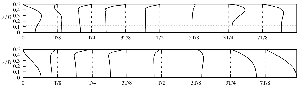
Figure 4: Snapshots of axial velocity profiles, taken at the free end of the pipe, at different phases of oscillation over one period T for (a) Re_{\max} = 2400 , \Lambda = 7.07 as an example of the high \Lambda regime and (b) Re_{\max} = 240 , \Lambda = 2.24 as an example of the low \Lambda regime. In the high \Lambda regime, all the profiles are essentially flat for r/D < 0.12 (marked with the fine dashed line) indicating little interaction between the Stokes layers on each side. In the low \Lambda regime, some profiles are essentially parabolic indicating each side is interacting.
