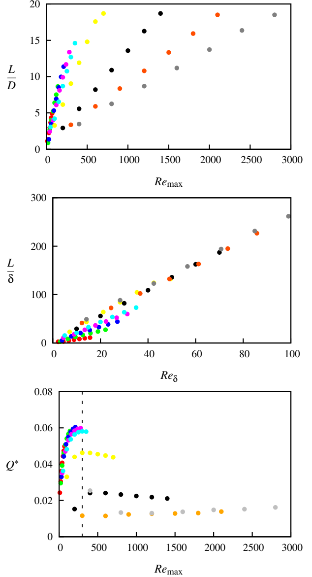
Figure 2: (a) Recirculation length L normalized by pipe diameter D as a function of Re_{\max} . (b) The same data as (a), but L is normalized by the Stokes layer thickness \delta . (c) Normalized flow rate as a function of Re_{\max} . The dashed line marks the value of Re_{\max} of the apparent optimum for flow rate. Colours of points represent values of \Lambda : \bullet , \Lambda = 1.12 ; \bullet , \Lambda = 1.58 ; \bullet , \Lambda = 1.94 ; \bullet , \Lambda = 2.24 ; \bullet , \Lambda = 2.50 ; \bullet , \Lambda = 3.54 ; \bullet , \Lambda = 5.00 ; \bullet , \Lambda = 6.12 ; \bullet , \Lambda = 7.07
