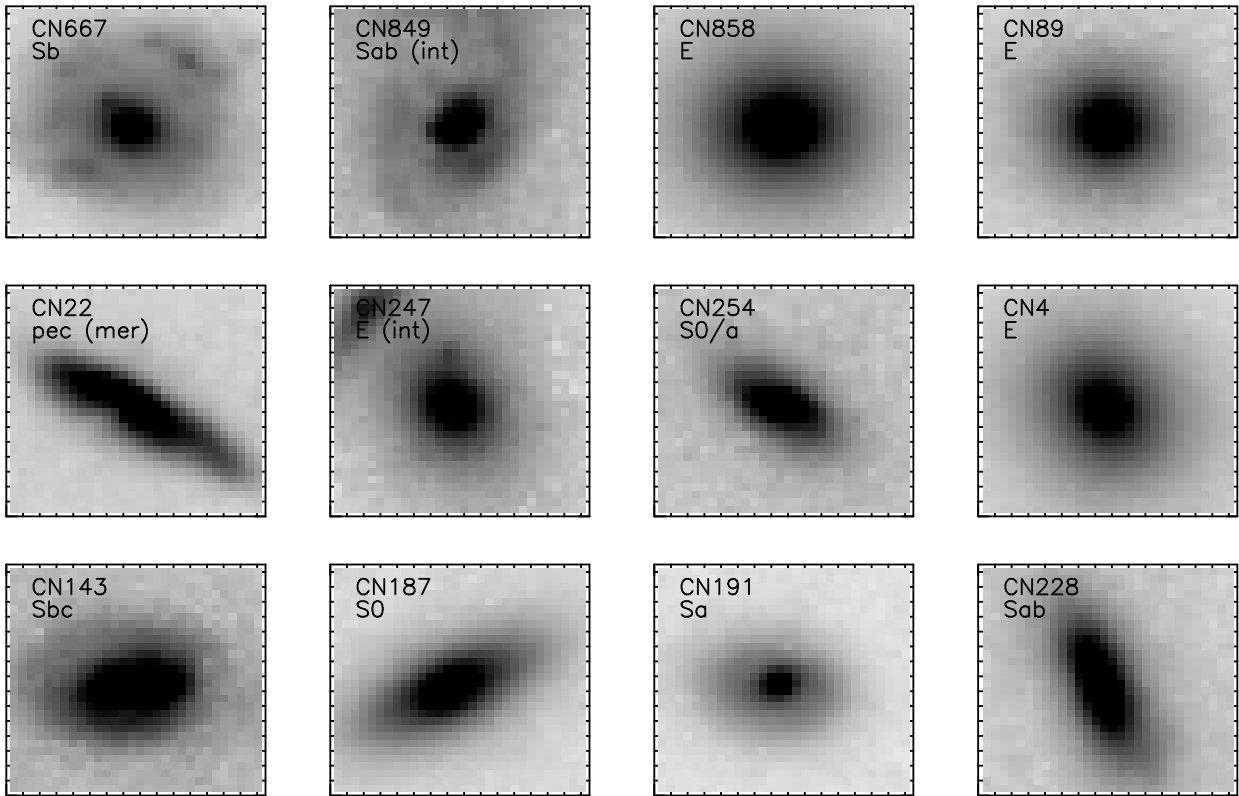
Figure 1. HST Wide Field Planetary Camera 2 (WFPC2) images of the E+A galaxy sample. Each image has dimensions 3'' \times 3'' , corresponding to approximately 13.8 kpc at the cluster redshift and comparable to the total IFU aperture.
