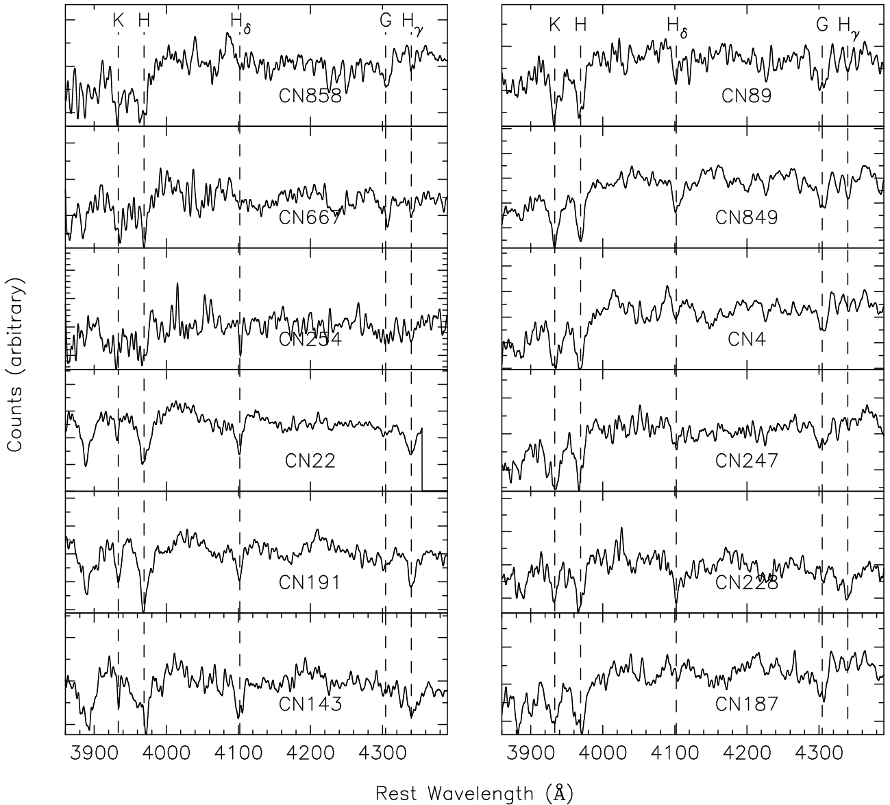
Figure 5. Spatially binned redshift-corrected spectra for the twelve galaxies in our E+A galaxy sample.
