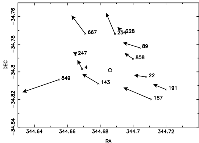
Figure 4. Vectors showing the magnitude and direction of the positional offsets of our target galaxies within the IFU's, as they appear on the sky. The lengths of the vectors have been scaled by a factor of 100 for display purposes. The circle indicates the centre of the FLAMES field of view
