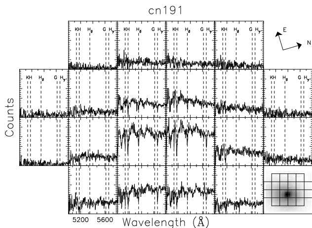
Figure 2. Spatial geometry of the IFU's used in our study. Each square represents an IFU lenslet, which is 0.5 on a side. The spectrum obtained through that lenslet (for CN191) is displayed within. The ordinate scale is identical in all lenslets; thus the continuum level reflects the level of light observed in that direction on the sky. Note the astrometric offset, which is discussed in Section 2.4. The bottom right panel shows the HST image of CN191 and its orientation with respect to the IFU.
