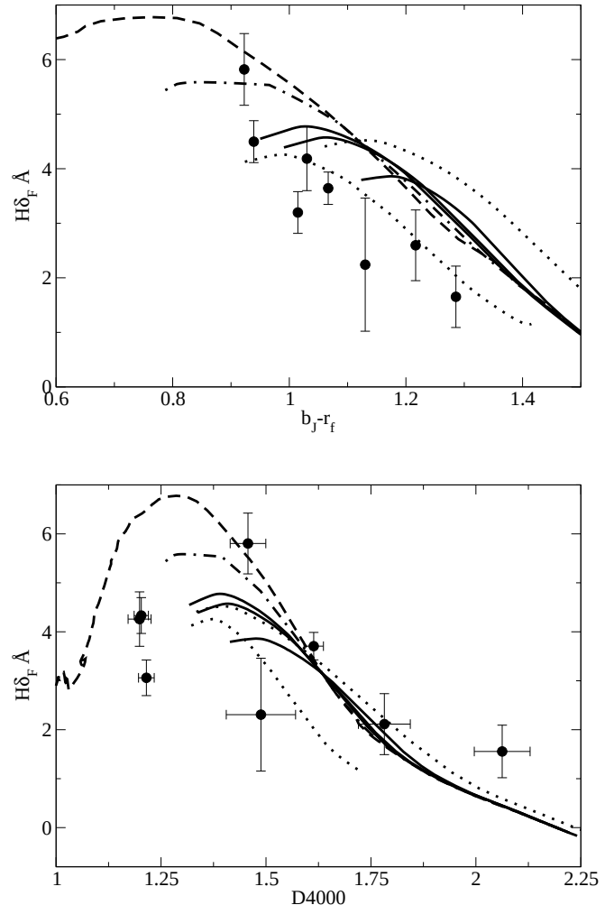
Figure 7. Top panel: H\delta_F plotted against b_J - r_f colour. The H\delta_F measurements from our sample are plotted as filled circles . The galaxy colours have been corrected for reddening (CS87) and K-correction. The curves are evolutionary tracks produced using the spectral synthesis models of Bruzual & Charlot (2003). The solid lines represent evolutionary tracks for models in which normal star formation is suddenly truncated. The dashed and dot-dashed lines show the evolution for a post-starburst galaxy. The dotted lines show the effect of varying metallicity. The details of these models are described in the text. Bottom panel: H\delta_F plotted against the D4000 index. The model curves are the same as those shown in the top panel.
