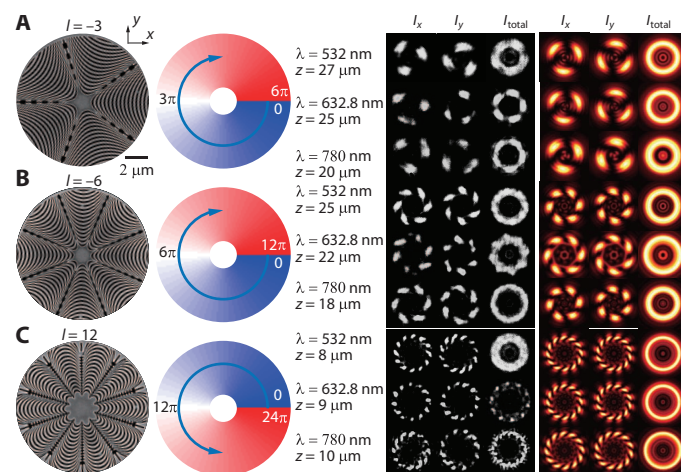
Fig. 2. OAM generators based on catenary arrays. (A to C) The topological charges for (A) to (C) are -3 , -6 , and 12 ( \sigma = 1 ), respectively. The first column represents the scanning electron microscopy (SEM) images of the fabricated samples. Scale bar, 2 \mu\text{m} . The second column shows the spiral phase profiles. The last two columns depict the measured (the third column) and calculated (the last column) results of I_x , I_y , and I_{\text{total}} for \lambda = 532 \text{ nm} (top row), 632.8 \text{ nm} (middle row), and 780 \text{ nm} (bottom row). The distances between the recording planes and the sample are indicated in each row.
