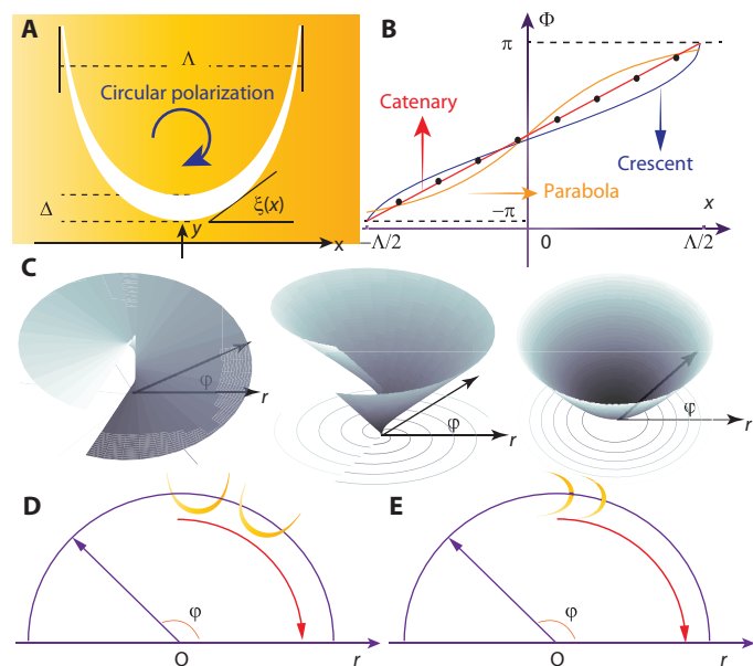
Fig. 1. Schematic representation of the geometric phase in optical catenaries. (A) Sketch map of a catenary aperture illuminated at normal incidence by CPL. Light is assumed to propagate along the +z direction throughout this paper. The inclination angle with respect to the x axis is denoted as \xi(x) . (B) Phase distributions of the catenary (red), parabola (orange), crescent (blue), and discrete antennas (black dot) for LCP illumination ( \sigma = 1 ). (C) Three typical kinds of phase profiles for the generation of pure OAM (left), HOBB (middle), and focused beam (right). (D and E) Arrangement diagrams of the catenary arrays for ordinary OAM (D) and HOBB or focused beam (E).
