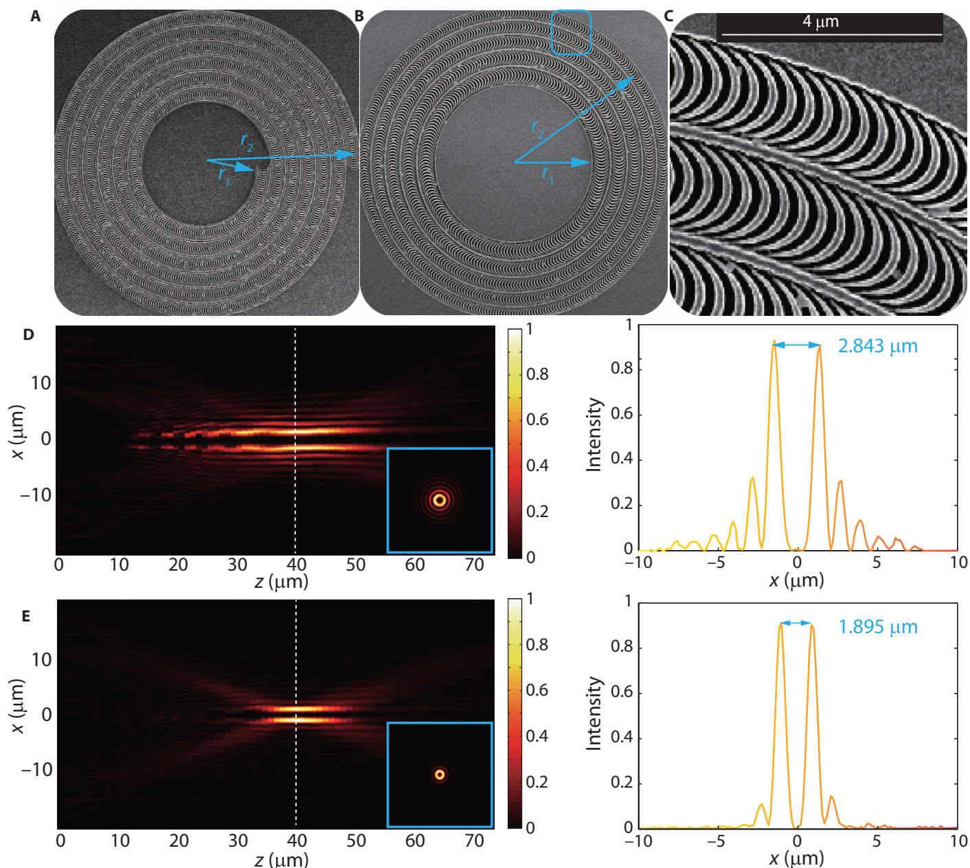
Fig. 4. Catenary arrays for the generation of HOB and focused OAM beam. (A and B) SEM images of the catenary arrays for HOB (A) and focused OAM (B). (C) Scaled view of the rectangular region shown in (B). (D and E) Measured cross-polarized intensity distributions of the HOB (D) and focused OAM (E) at a wavelength of \lambda = 632.8 nm for RCP illumination ( \sigma = -1 ). The intensities at the xy plane ( x, y \in [-20, 20] \mu\text{m} , z = 40 \mu\text{m} ) are plotted in the insets.
