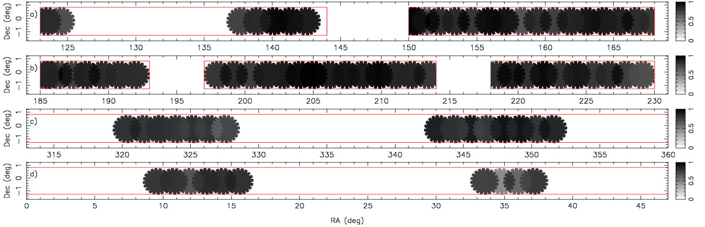
Figure 20. The 2SLAQ spectroscopic completeness mask, defined as the fraction of observed priority 5 and 6 objects which have high quality identifications (ID quality = 1). The grey-scale extends from 0.0 (white) to 1.0 (black). The regions plotted are the same as in Fig. 19.
