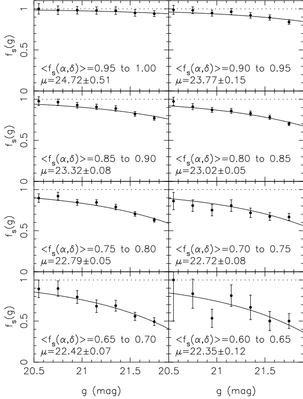
Figure 21. The 2SLAQ spectroscopic completeness as a function of g -band magnitude for sectors with different mean completeness values, \langle f_s(\alpha, \delta) \rangle . In each case the best fit magnitude-dependent completeness model (Eq. 8) is shown (solid line).
