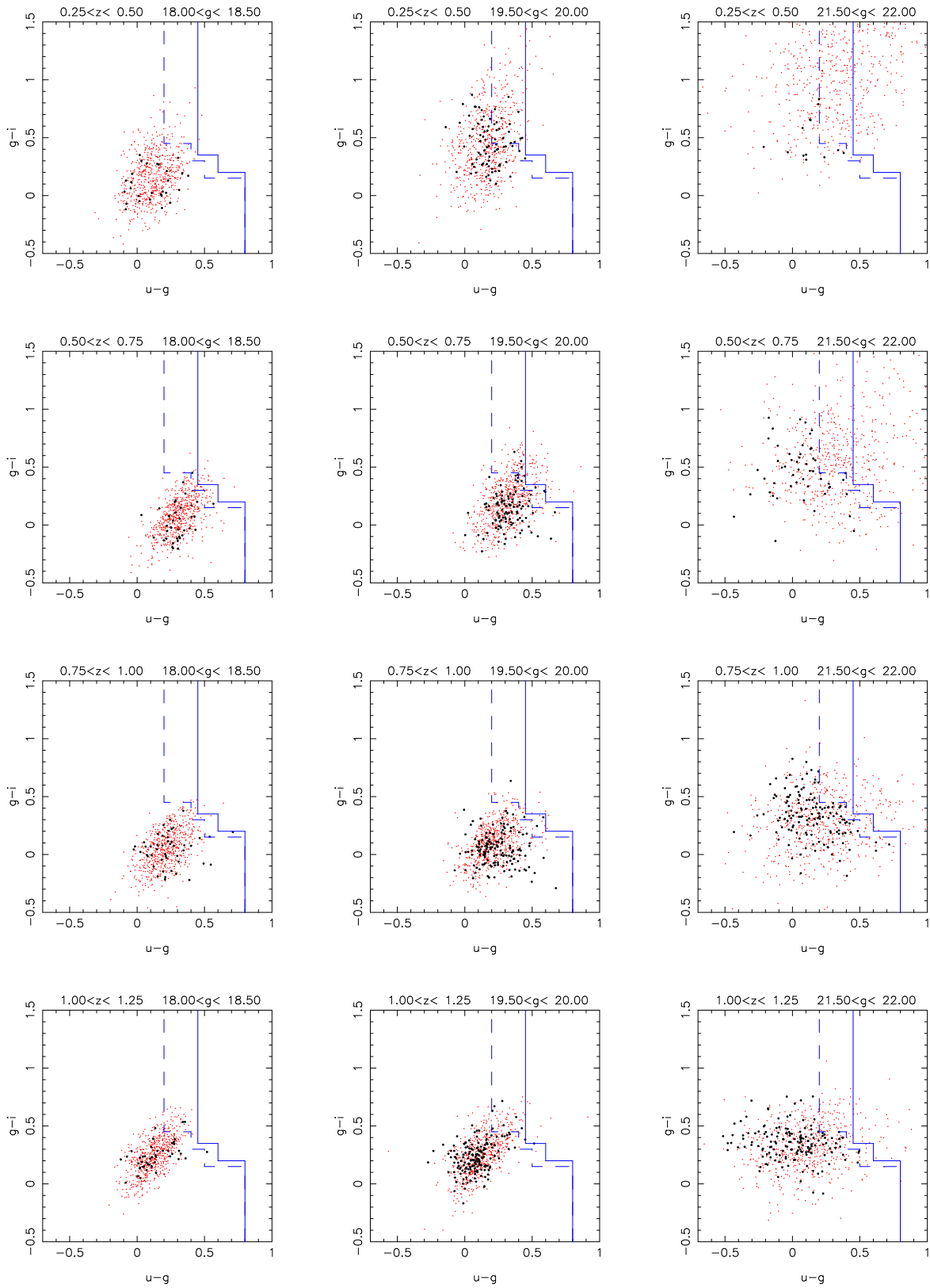
Figure 12. A comparison of 2SLAQ (black points) and simulated (red points) u - g and g - i colours in the redshift intervals 0.25 < z < 0.50 , 0.50 < z < 0.75 , 0.75 < z < 1.00 and 1.00 < z < 1.25 (top to bottom). We compare these distributions as a function of g -band magnitude in \Delta g = 0.5 mag bins with 18.0 < g < 18.5 , 19.5 < g < 20.0 and 21.5 < g < 22.0 (left to right). The blue lines indicate the QSO selection limits at g < 21.15 (solid line) and g > 21.15 (dashed line). Both the data and simulated points show a reddening of the g - i colour and increased scatter towards fainter magnitudes. The simulated points are a realization of model 2 from Table 11, which provides one of the better matches to our data.
